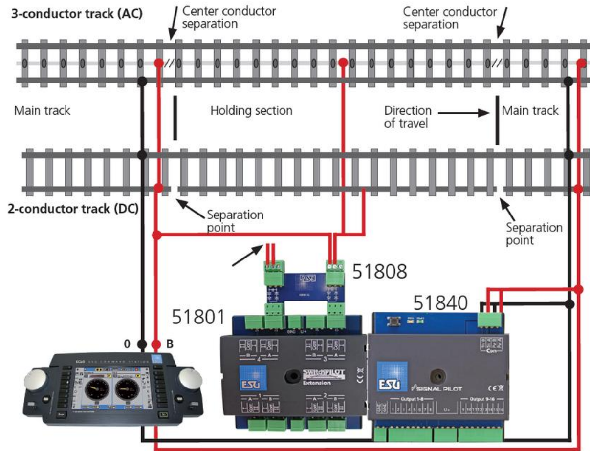
Figure 8: Switch the ABC braking section with SignalPilot and SwitchPilot Extension
