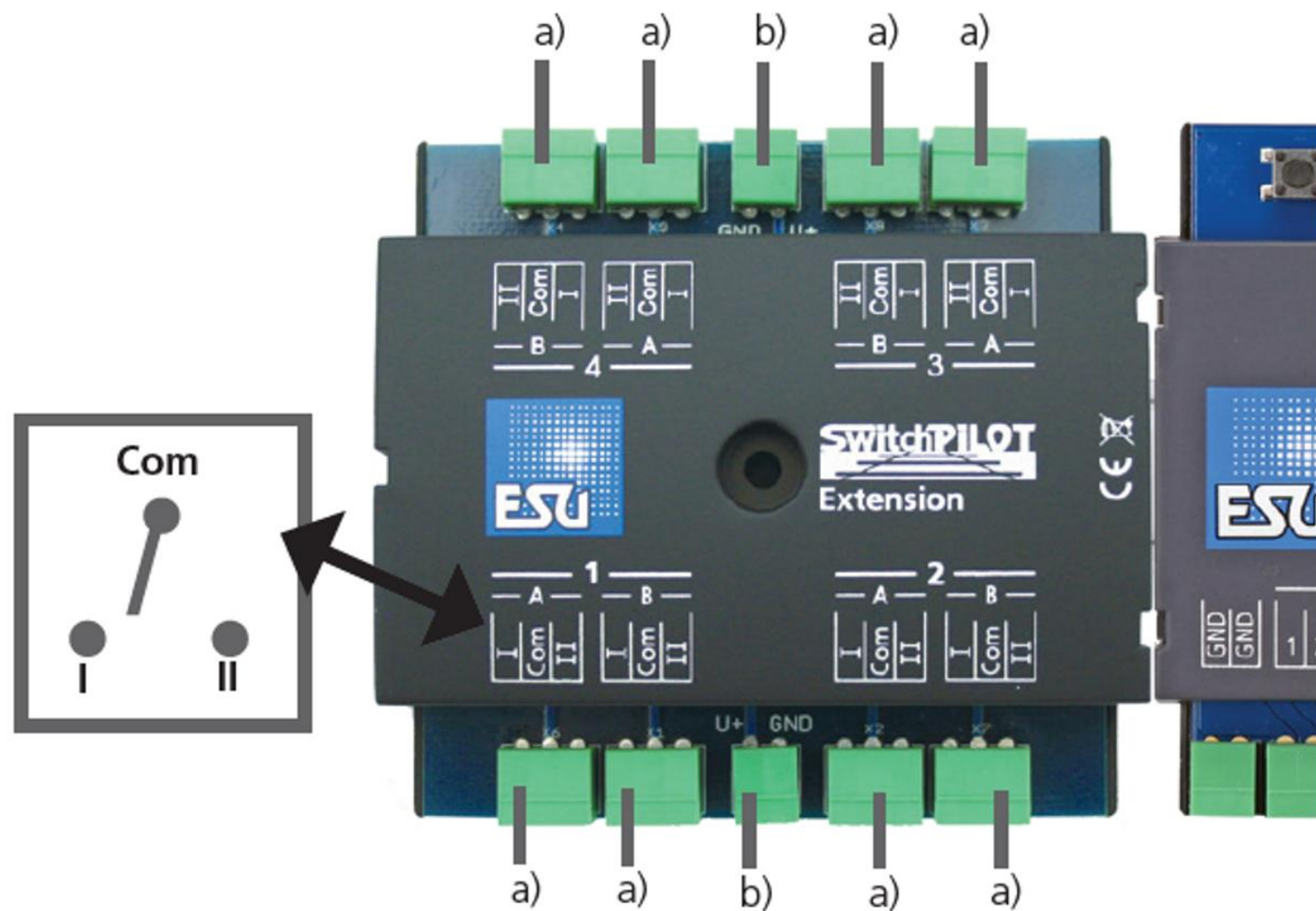
Figure 6: SignalPilot with mounted SwitchPilot Extension
